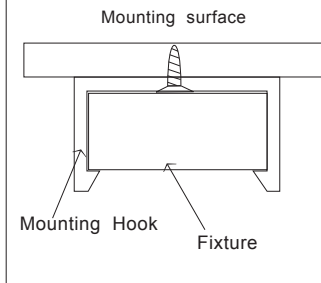
Figure 3 (Completed installation)
